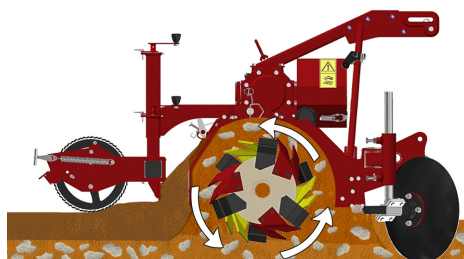
Soil preparation principle
