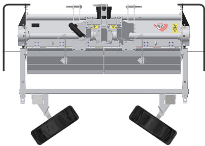
Option DCE 250 : Retractable wheels for road transport
