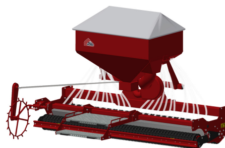
Pneumatic seeder
