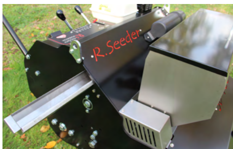
Calibration drawer
